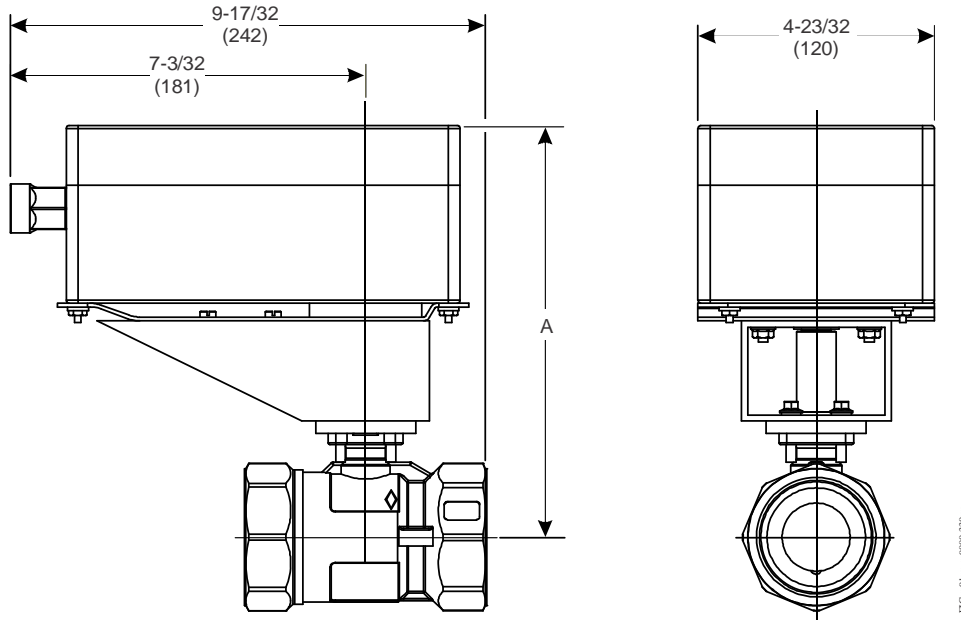
Figure 15: Non-Spring Return VA9104 and M9106 Series and Spring Return VA920x Series Actuated VG1241, VG1245, VG1841, and VG1845 Series Ball Valve and Field Installed M9000-341 Weather Shield Dimensions, in. (mm)
